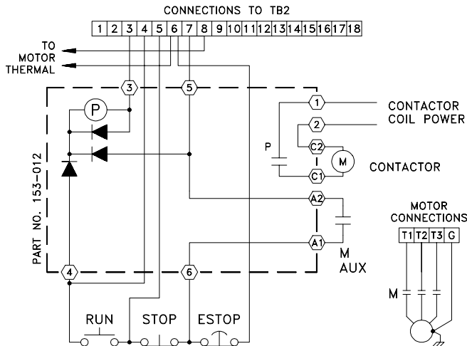
Figure 15: Connecting an output contactor with an externally powered coil to a Model 4000.
