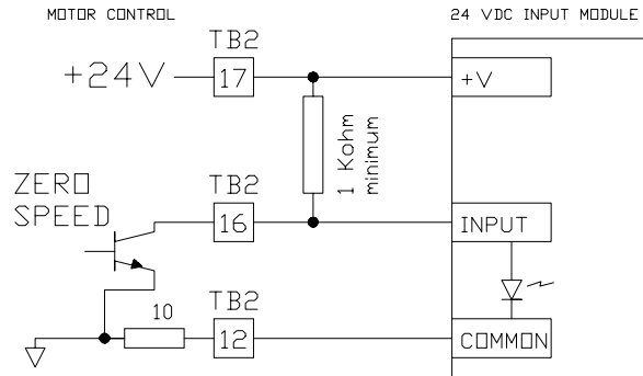
Figure 25: SOURCING connection to a PLC.
