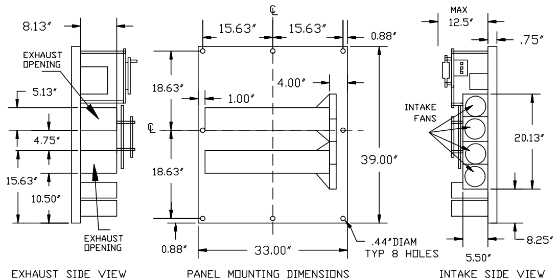
Figure 11: The mounting dimensions of the chassis version of Model 4000.
