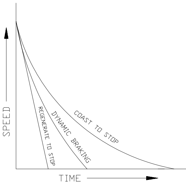
Figure 2: Stopping methods for motors compared.
