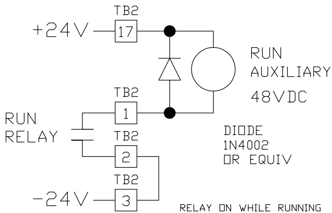
Figure 19: Connections to add an auxiliary RUN relay to the control.
