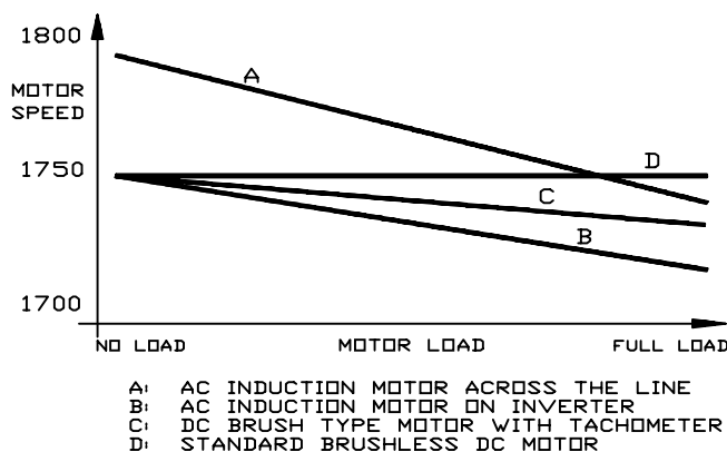
Figure 1: Comparison of speed regulation of typical industrial motors from no load to full load.
