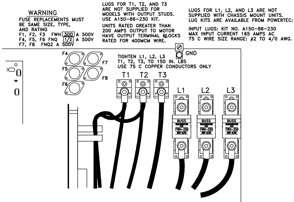
Figure 14: Input power fuses and output connections of the Model 4000..
