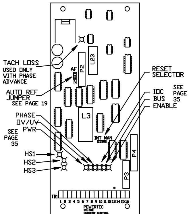
Figure 32: Major parts of the 141-108 Current Controller board.
