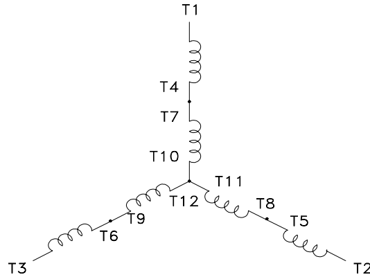
Figure 5: Single-wye connections for a Brushless DC motor.
