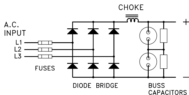
Figure 3: Simplified drawing of input power section of a Brushless DC motor control.
