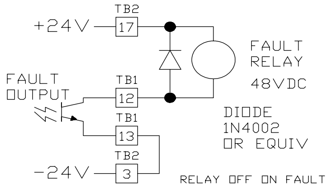
Figure 20: Adding a FAULT relay.
