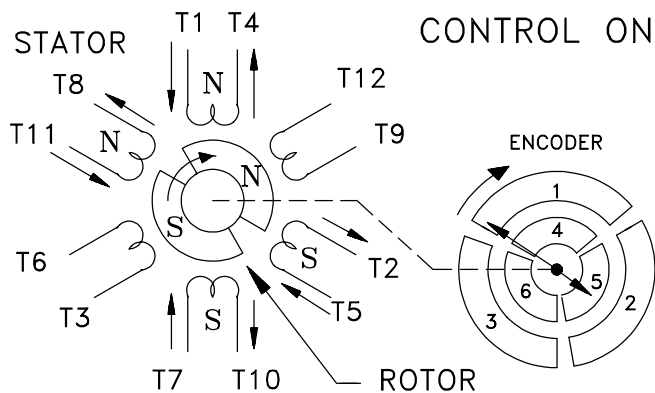
Figure 7: Current flows in the stator of the motor after the control is turned on in the position shown.
