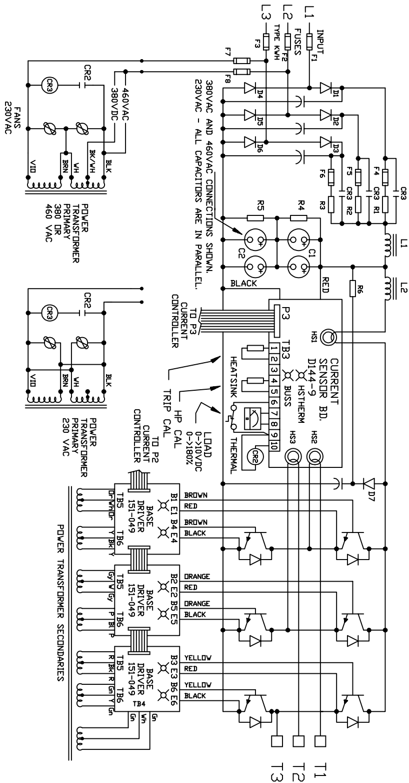
Figure 28: Simplified schematic drawing of the Model 4000 power circuits.
