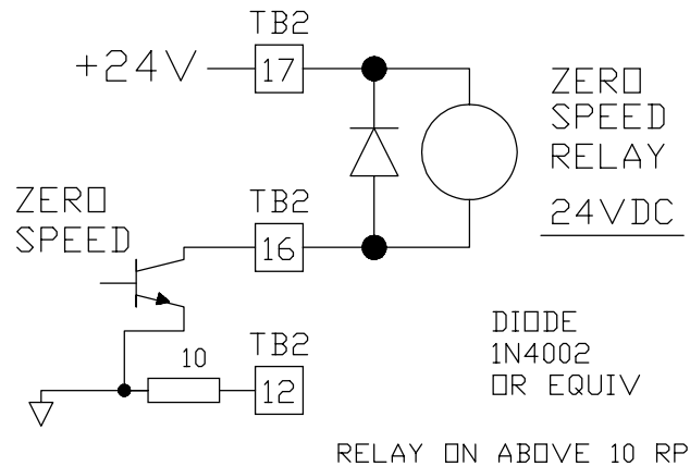
Figure 22: Connecting a ZERO SPEED relay. Note that the relay coil is 24VDC, so current should be kept low.
