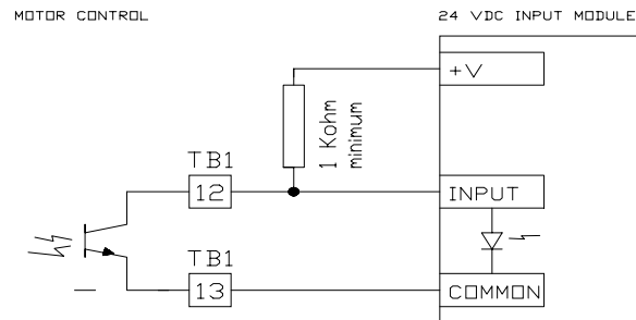
Figure 26: Connecting FAULT output to a PLC.
