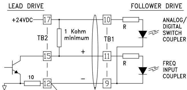
Figure 18: Connections for any other POWERTEC Brushless DC drive (except the Model 500) to follow a Non-regenerative drive at a 1:1 ratio.
