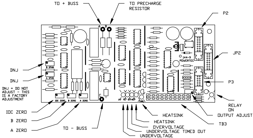
Figure 29: Parts layout and important points on the Current Sensor board 144-9.
