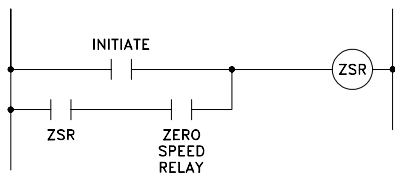
Figure 23: A circuit to eliminate chatter on the zero speed relay.
