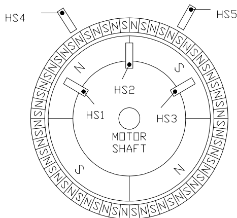
Figure 9: The encoder assembly - four magnets indicate position; outer magnets indicate speed and direction.
