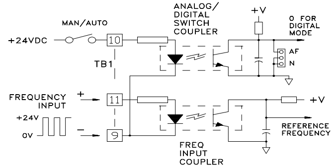
Figure 16: Analog/digital switch and frequency input circuits of the POWERTEC Brushless DC motor control.
