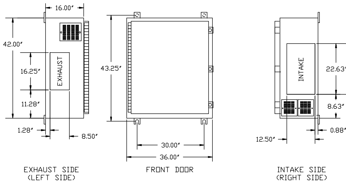
Figure 12: Physical dimensions of the NEMA 1 version of the POWERTEC Model 4000.
