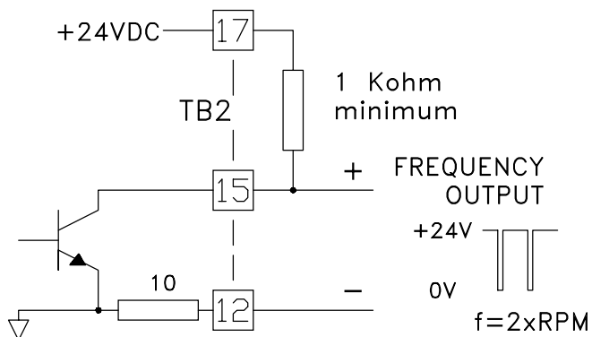
Figure 17: Connections for the frequency output of the Non-regenerative drive.
