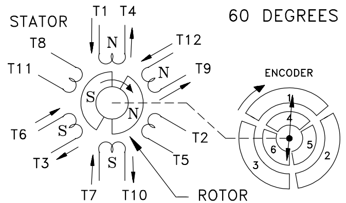
Figure 8: When the motor rotates 60 degrees the encoder switches the output transistors to rotate the field.
