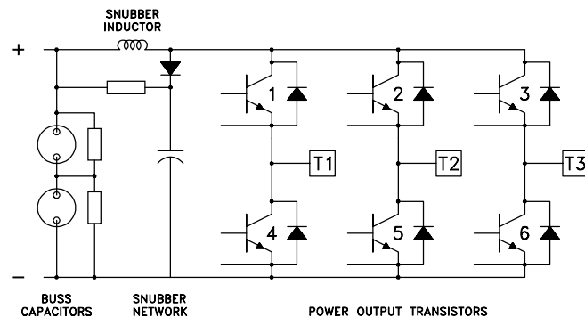
Figure 4: The power output bridge consists of six power transistors and associated snubber components.
