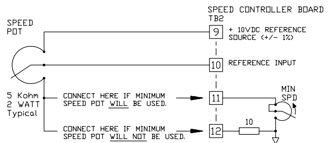
Figure 27: Connections for using or not using a minimum speed pot with the Model 4000.
