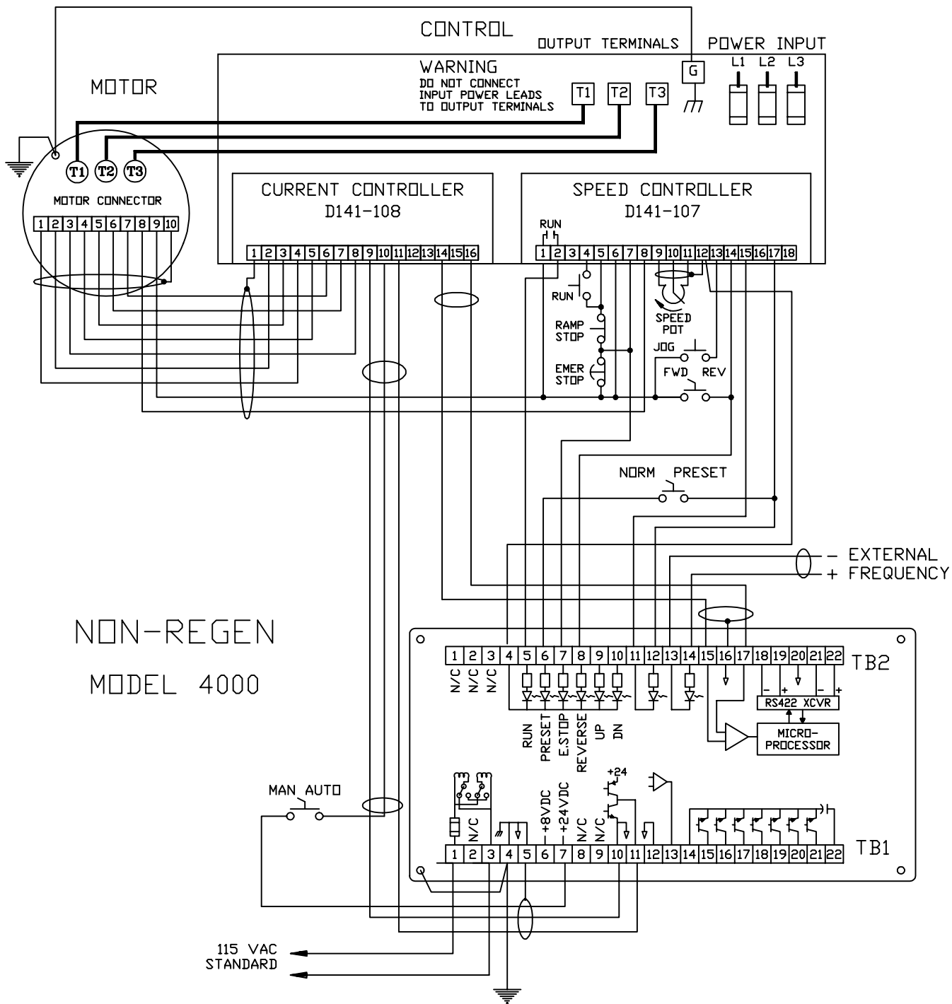
Figure 35: Connections of the Model 4000 to the optional POWERTEC DIGIMAX IV .
