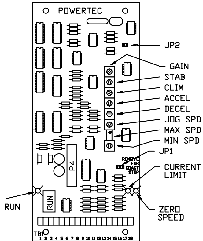
Figure 33: Major parts of the 141-107 Speed Controller board.
