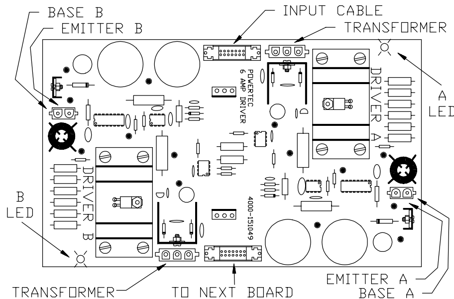
Figure 30: Layout and connections of the Base Driver Board 151-049.
