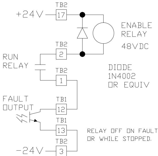
Figure 21: Obtaining an ENABLE indication.
