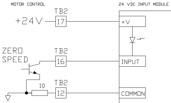
Figure 24: SINKING connection to a PLC.
