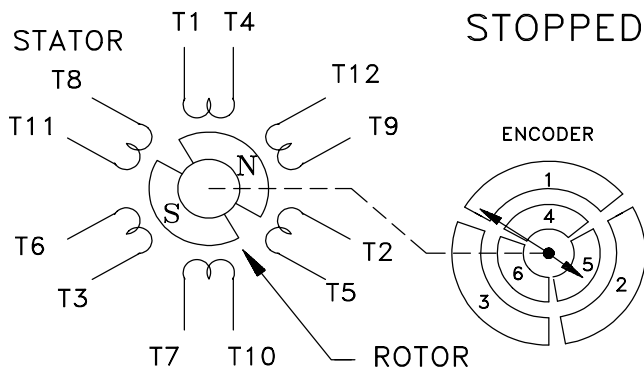
Figure 6: Simplified drawing of the major parts of the Brushless DC motor.
